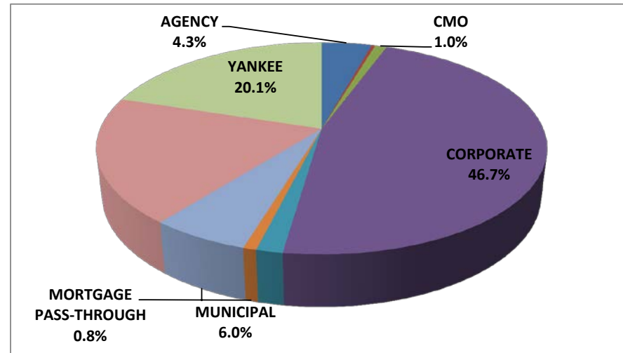
Sectors By % 3
